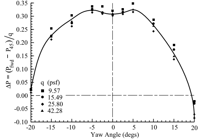
Figure 8. Yaw differential pressure normalized by dynamic pressure (P_{fwd}-P_{45})/q .
