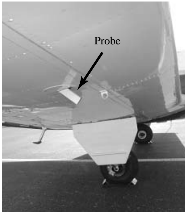
Figure 1. Angle of attack probe mounted under the wing.
